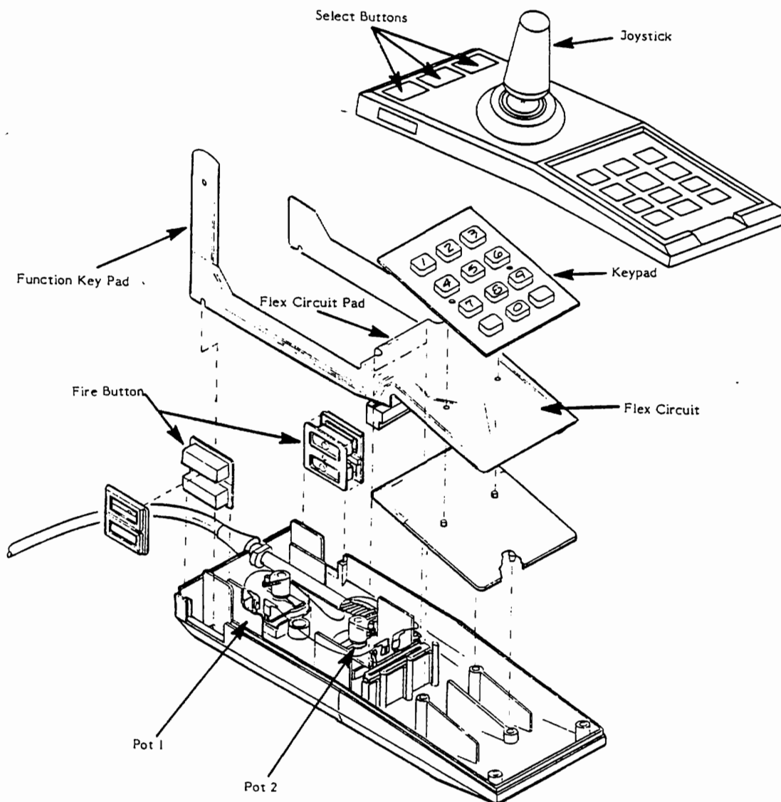
Figure 6-1. Model 5200 Game Controller.
