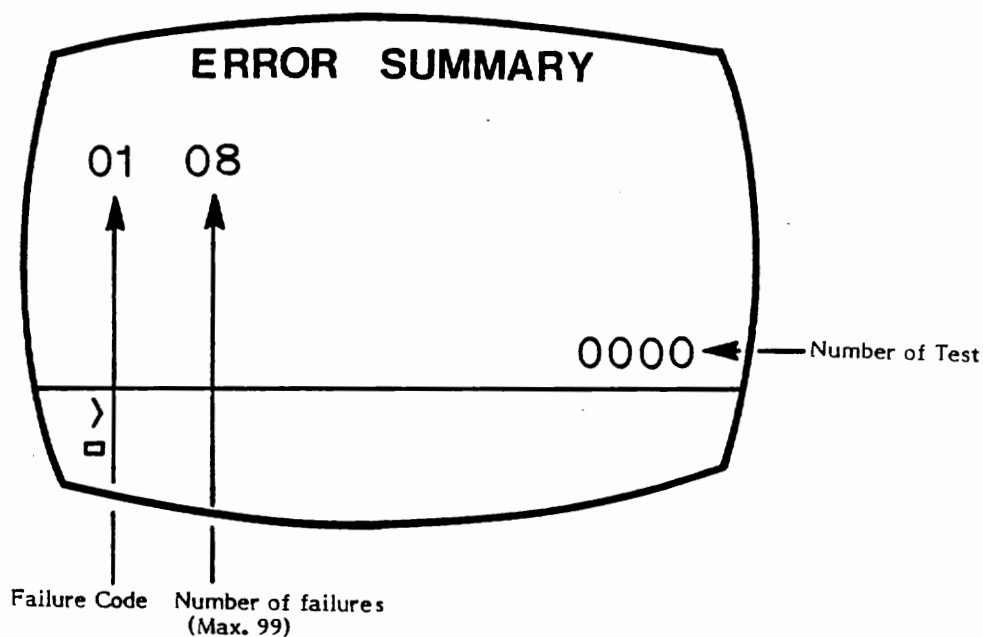
Figure 3-5. Error Summary.
