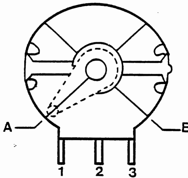
Figure 6-4. Pot and Arm Assembly
