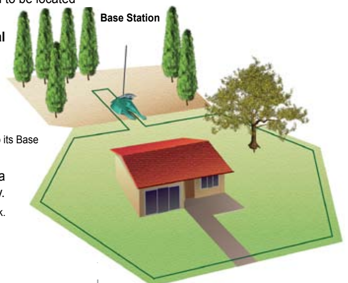
Option B - External setup (Outside the lawn)
